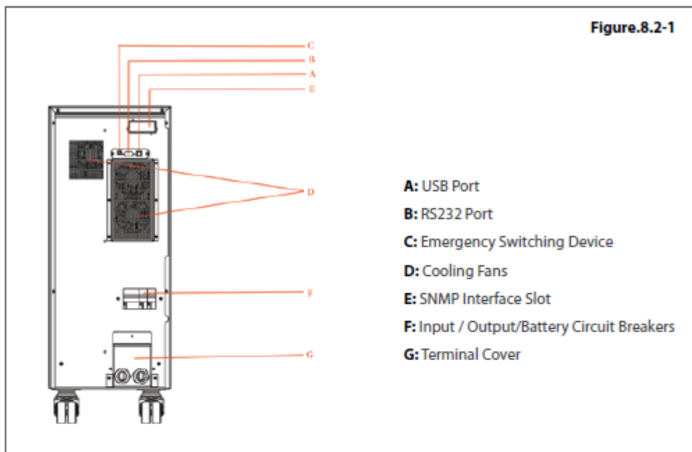
Keor S 3kVA without Transformer
